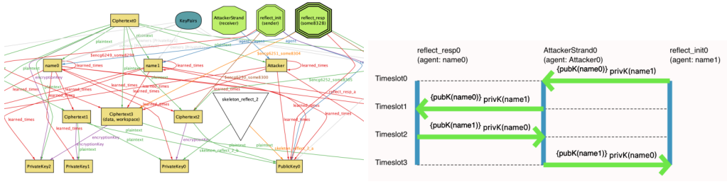
Fig. 4. Visualizing the example protocol. Left: Alloy with projection. Right: custom visualization via a sequence diagram. The middle agent in the diagram represents the medium of communication which, following Dolev and Yao [1983], is synonymous with the attacker.
