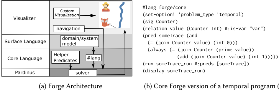
Fig. 8. Forge consists of several layers. Its languages compile to a common core.
