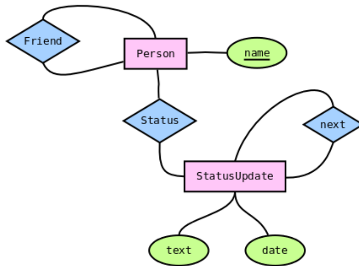
Figure 4.5. Social network data model
