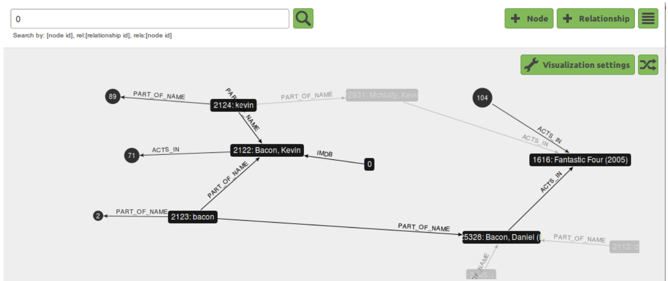
Figure 26.4. Browsing and manipulating data
