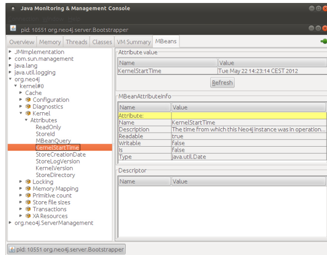
Figure 25.2. Neo4j MBeans View
