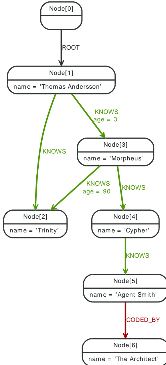
Figure 27.1. Shell Matrix Example
