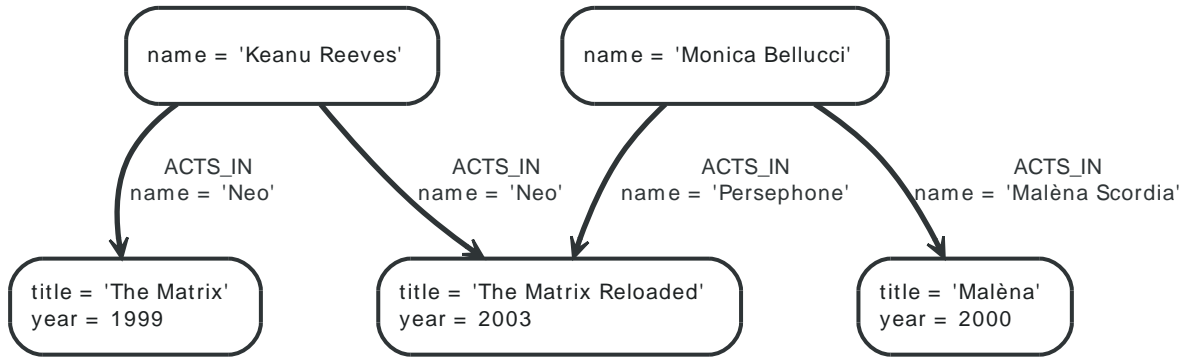
Figure 14.1. Movie and Actor Graph
