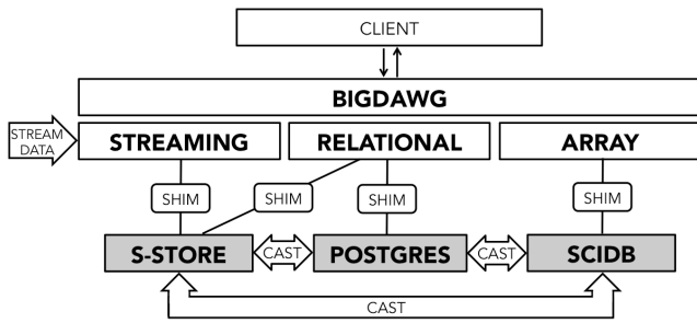
Fig. 1. BigDAWG 1.0 Architecture
