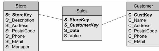
Fig. 3. Sample sales data warehouse schema
