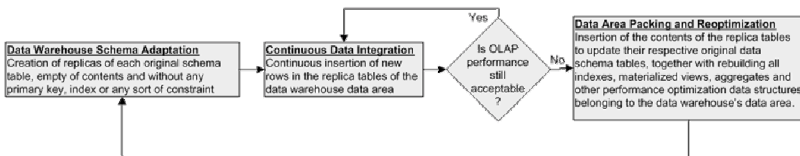
Fig. 2. General architecture of the proposed continuous data warehouse loading methodology
