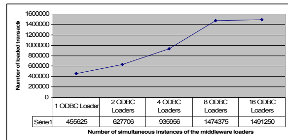
Fig. 1. ODBC insertion volume for running simultaneous data loading middleware instances
