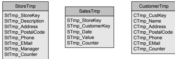
Fig. 4. Sample DW sub-schema for supporting useful-time DW
