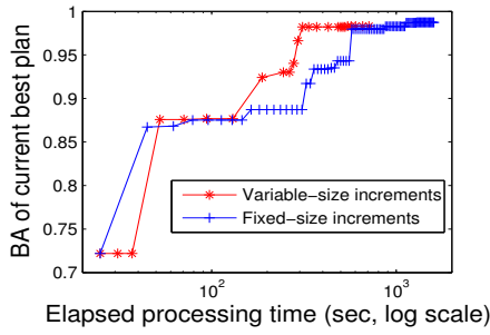
Figure 6: Choosing chunk sizes (Periodic-large-tb, \Delta=30 in Fig. 3)
