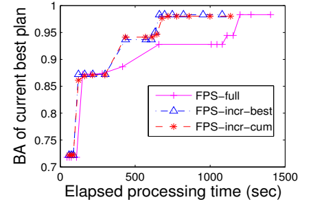
Figure 11: Improvements with sharing (Periodic-large-tb)
