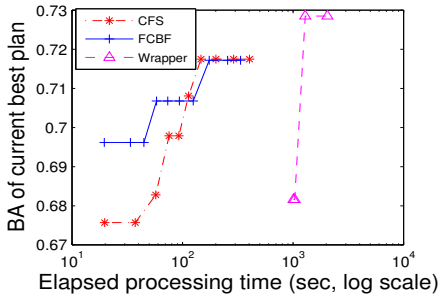
Figure 7: Comparing attribute-selection techniques (Aging-real)
