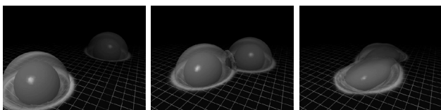
Figure 1. The ASC project investigates astrophysical phenomena involving strong dynamic gravitational fields such as this grazing collision of two neutron stars. The surfaces represent the density of the stellar matter while the warping of the gridded surface represents the gravitational flux on the plane of the collision.
