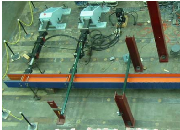
Figure 7: The physical substructure test at the University of Colorado
