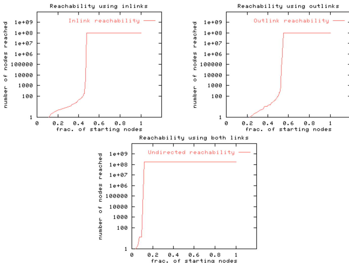
Figure 7: Cumulative distribution on the number of nodes reached when BFS is started from a random node. Figure (a) follows in-links, (b) follows out-links, and (c) follows both in and out links. Notice that there are two distinct regions of growth, one at the beginning and an "explosion" in 50 % of the start nodes in the case of in- and out-links, and for 90% of the nodes in the undirected case. These experiments form the basis of our structural analysis.
