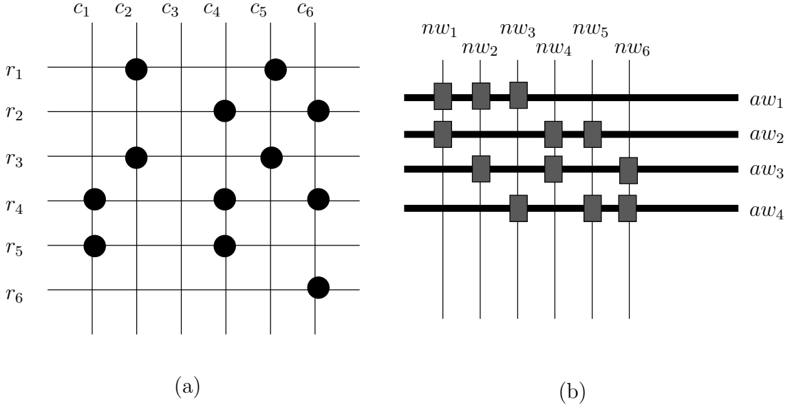
Figure 1: (a) A nano-array and (b) 2-hot addressing of six nanowires \{nw_1, \dots, nw_6\} with four micro-level address wires \{aw_1, \dots, aw_4\} . In practice the microwires would be much larger than the nanowires.
