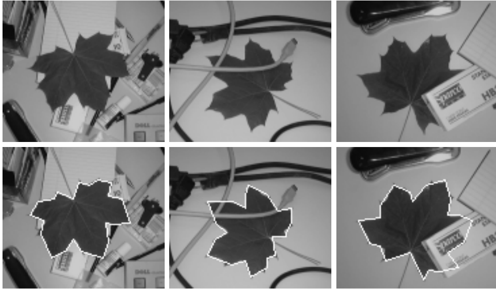
Figure 12: Matching the maple leaf model to different images.
