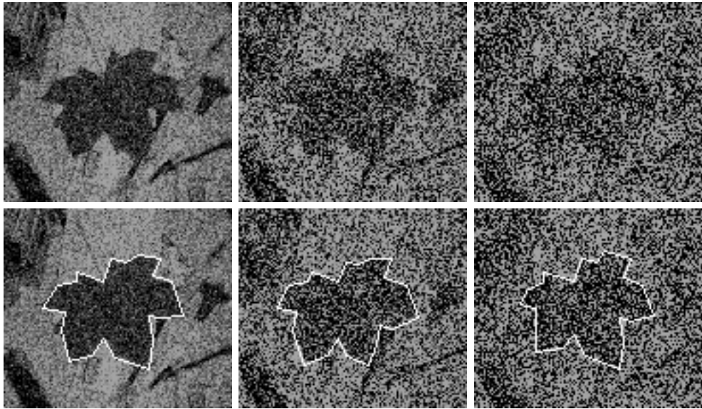
Figure 14: Matching to an image corrupted by increasing amounts noise.
