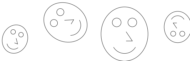
Figure 8: Different objects with the same shape.
