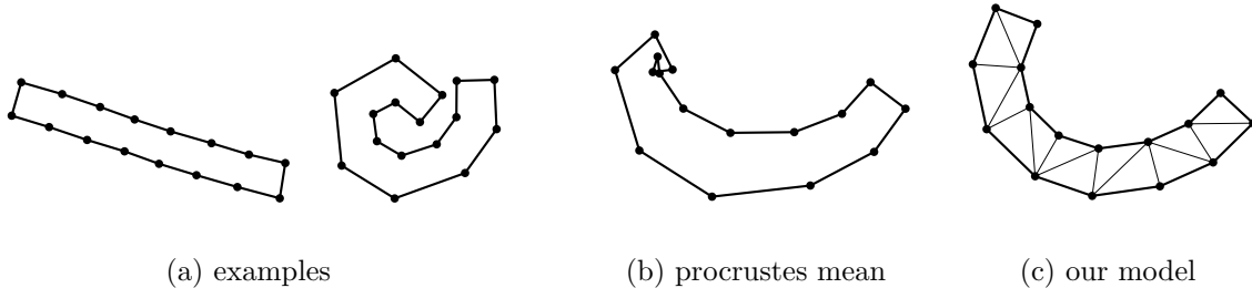
Figure 16: Comparing the procrustes mean and triangulated model for the two input polygons shown in (a). Procrustes analysis breaks down when the samples can not be aligned using similarity transformations (b), while our model is good (c).
