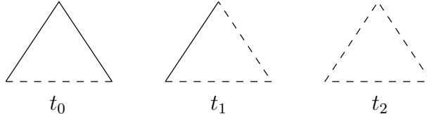
Figure 6: Different triangle types. The first triangle type corresponds to ends of branches, the second type corresponds to branches and necks while the last corresponds to connections between multiple branches and necks.
