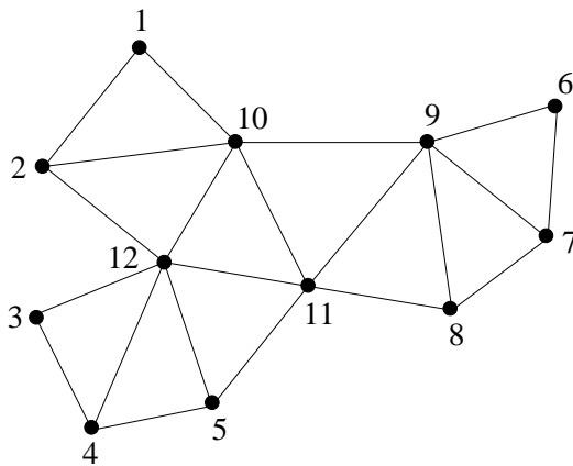
Figure 9: Perfect elimination scheme for the vertices of a triangulated simple polygon.
