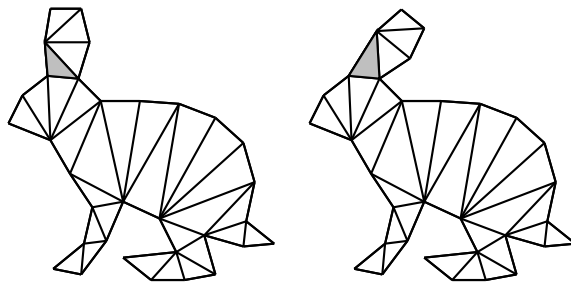
Figure 7: The rabbit ear can be bent by changing the shape of a single triangle.
