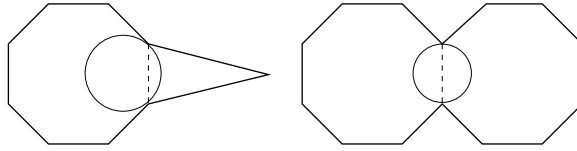
Figure 5: Limbs and pinch points are naturally represented in the CDT. These pictures show the defining circle for a diagonal that corresponds to a limb boundary and a diagonal that corresponds to a pinch point.
