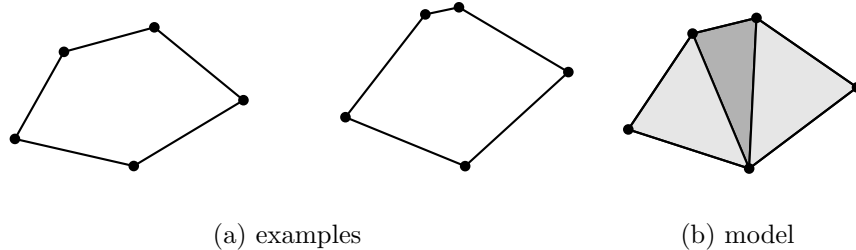
Figure 2: Two examples of a deformable object (a), and the learned model (b). The color of each triangle in the model indicates how much their shapes vary across different examples (darker triangles vary more).
