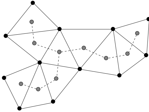
Figure 4: The graphical structure of the triangulation, G_T , is shown with black nodes and solid edges while the dual graph, D_T , is shown with gray nodes and dotted edges.
