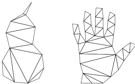
Figure 3: Pear, and hand represented by triangulated polygons. The polygonal boundaries represent the outlines, while the triangulations decompose the objects into parts.
