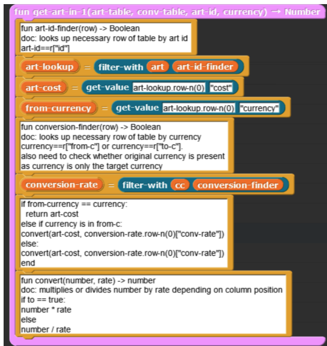
Figure 5: A student plan with code in blocks
