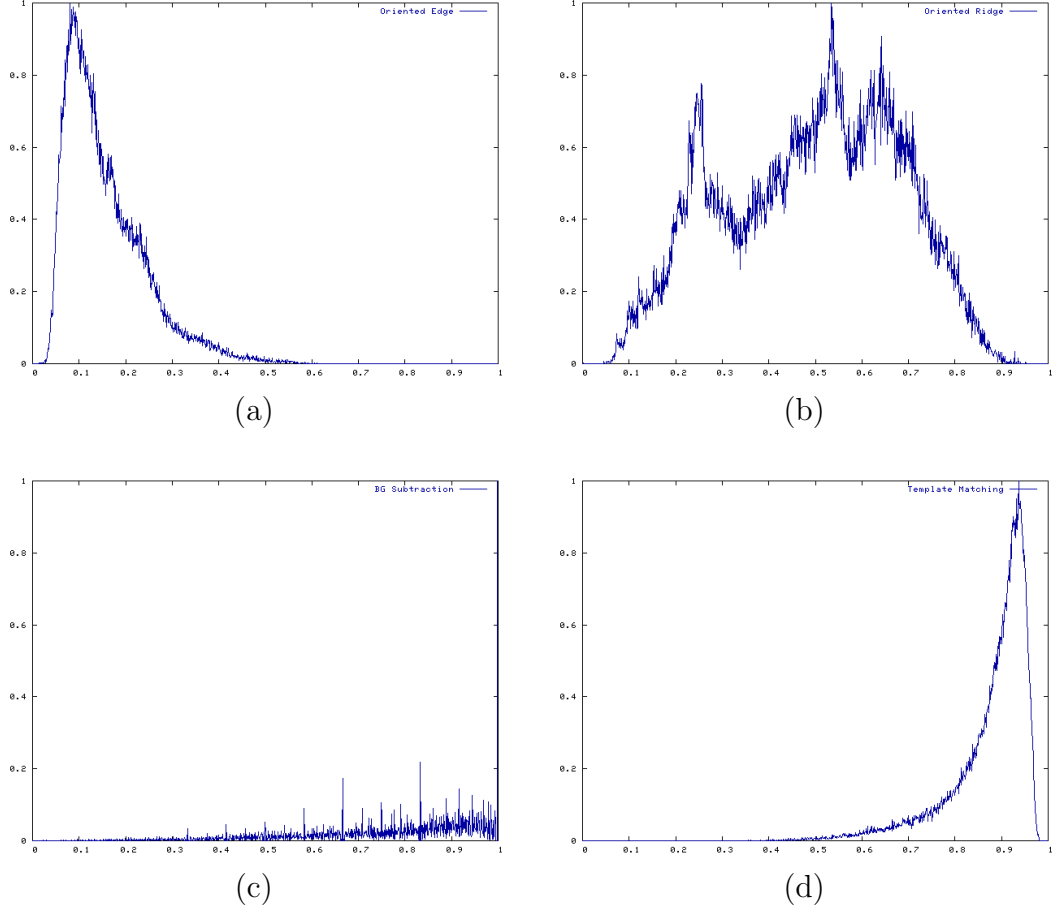
Figure 3.1: Measurement function histograms: Plots (a), (b), (c), and (d) represent the measurement function histograms for oriented edge detection, oriented ridge detection, background subtraction, and template matching respectively. These histograms were constructed after tracking three frames with 1000 particles.
