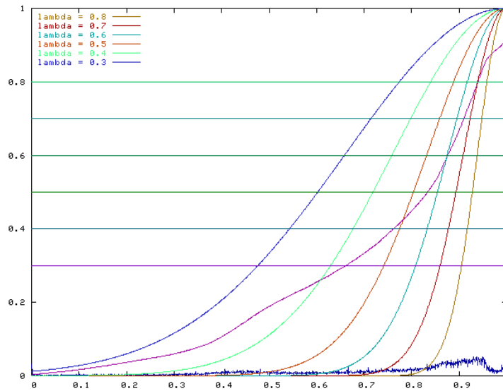
Figure 3.2: Variance with respect to \lambda : The non-decreasing function (shown in both plots) represents the cumulative plot of the measurement histogram values. The relationship between \lambda and \sigma can be seen in the plot above. The successively smaller Gaussian distributions correspond to \lambda values of 0.3, 0.4, 0.5, 0.6, 0.7, and 0.8. The horizontal lines corresponding to each \lambda value intersect the cumulative plot directly above the domain value \sigma measurement units from the mean \mu = 1.0 .
