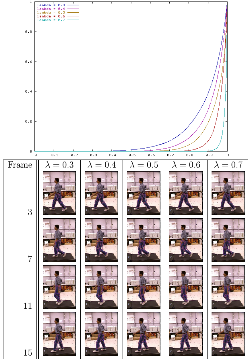
Figure 4.4: Template matching tracking results with respect to \lambda : The distributions (top) are plotted according to the specifications in Section 4.2.1.
