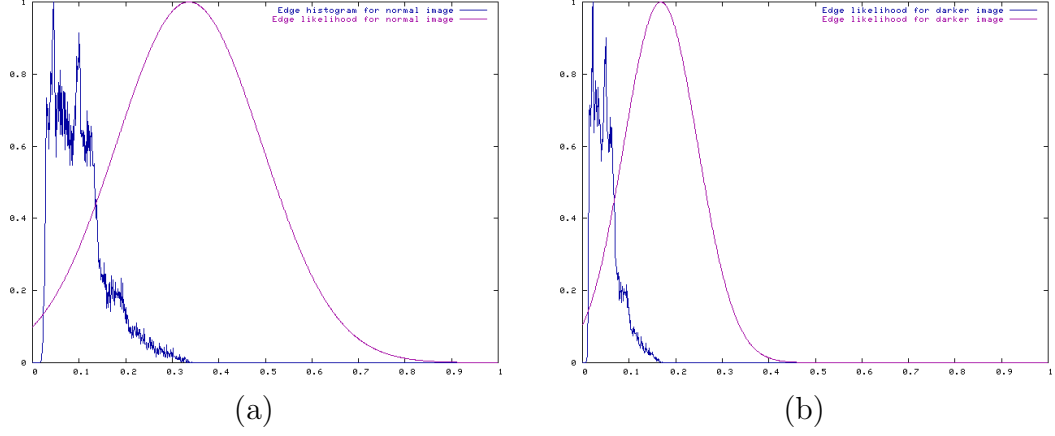
Figure 3.3: Oriented edge variance with respect to image brightness: The domain in these plots are measurement values. The jagged plots are oriented edge measurement histograms, and the Gaussians are likelihoods — conditioned on the measurement histograms — for given measurement values. The plot in (a) shows the likelihood mapping for the oriented edge measurement given our normal test sequence as input. The plot in (b) shows the same distribution when the input images have half of their original brightness. The mean and variance dynamically adjust to the change in image statistics; the edges in the darker image will be less pronounced in the measurement function, but the oriented edge likelihood will not be affected.
