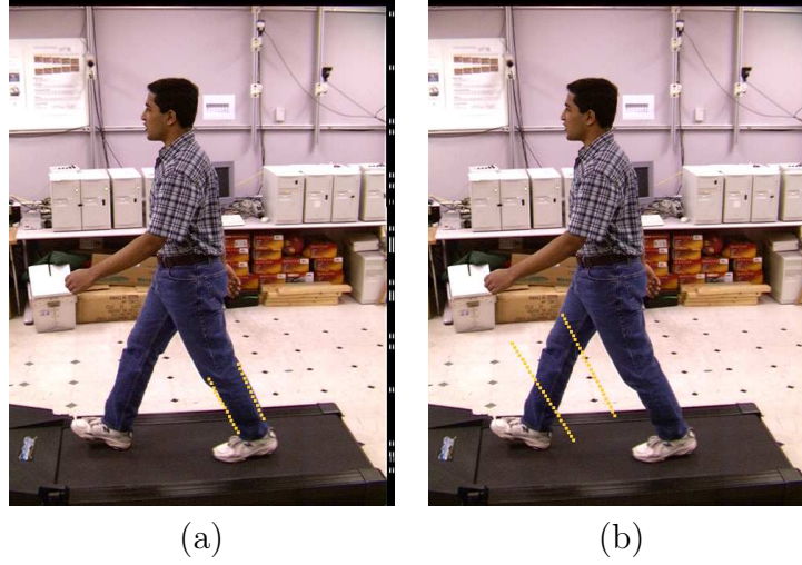
Figure 2.5: The constancy of measurement frequency in one-dimensional image space: Both (a) and (b) show the actual pixel locations of the individual oriented edge sub-measurements for a limb parameterized further and closer to the camera respectively. The number of samples taken in the image per unit distance is constant.
