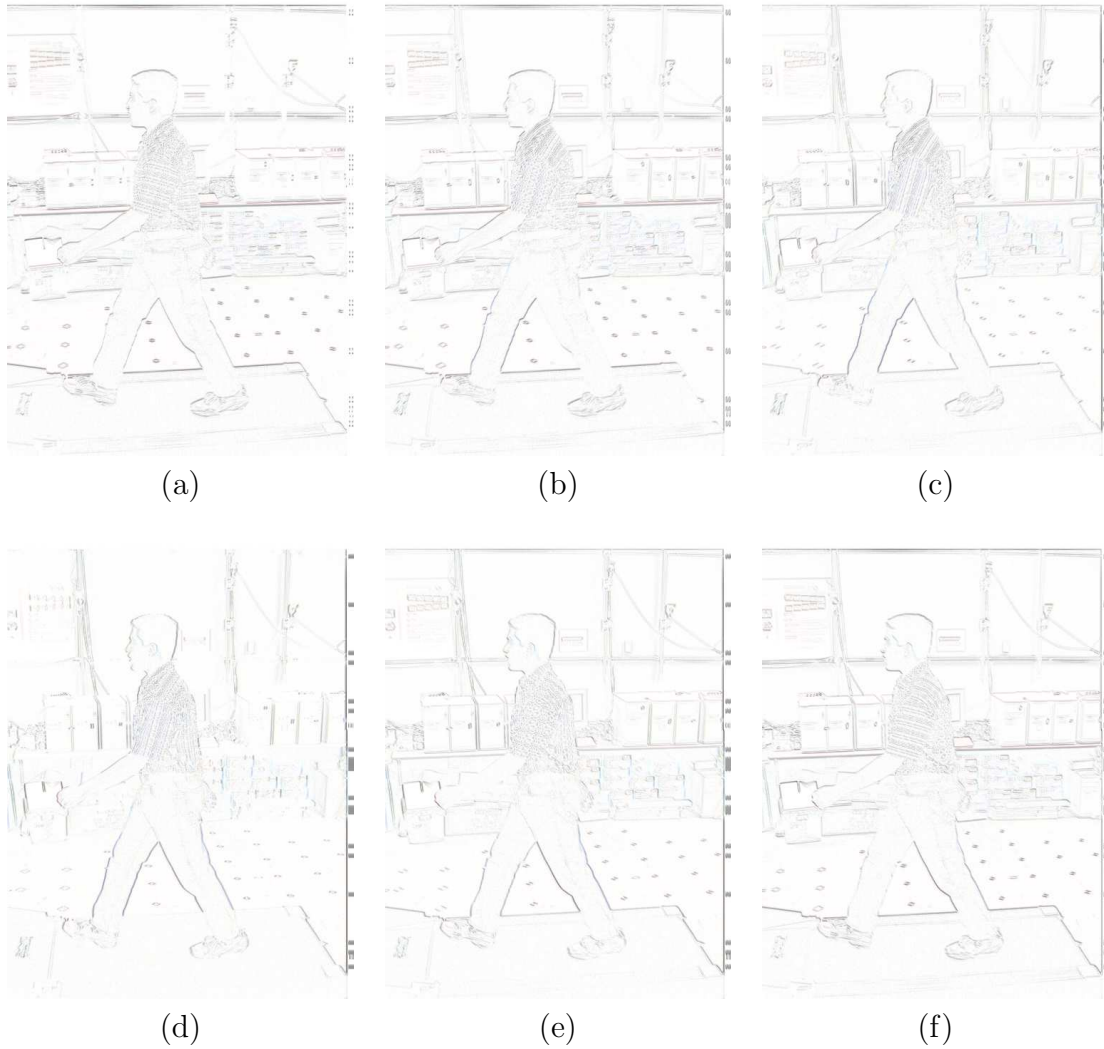
Figure 2.4: Oriented edge detection: Images (a) through (f) demonstrate oriented edge measurements at the lowest pyramid level given an identical source image and a changing parameter \theta . (The pixel intensities are negated for printability) Specifically, \theta = \{0, \frac{\pi}{3}, \frac{2\pi}{3}, \pi, \frac{4\pi}{3}, \frac{5\pi}{3}\} in the images (a) through (f) respectively.
