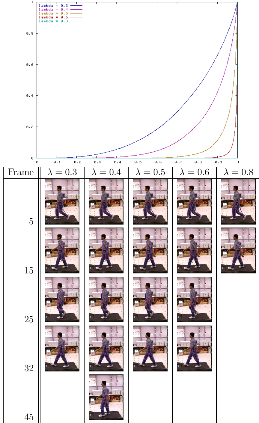
Figure 4.3: Background subtraction tracking results with respect to \lambda : The distributions (top) are plotted according to the specifications in Section 4.2.1. The tracking results were generally equivalent for \lambda > 0.4 , though the eccentricities for the higher \lambda values would prohibit robust tracking with multiple measurement models.
