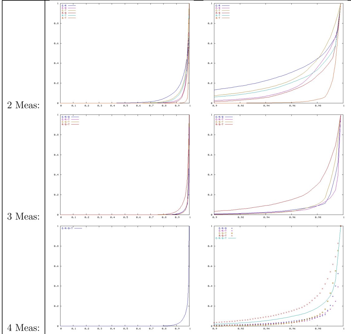
Figure 4.8: The effect of measurement combinations on the posterior distribution: The cumulative plots of the posterior distributions become more eccentric as additional measurement criteria are considered. Note that for measurements which are increasingly dependent probabilistically, the cumulative distribution is especially eccentric. (E.g., background subtraction and template matching) The magnified (right) cumulative plot for the posterior distribution after using 4 measurements is given context by the plots for 3 measurements.
