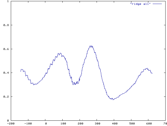
Figure 2.6: Oriented ridge measurement results: The plot corresponds to oriented ridge measurement values gathered along the path illustrated in Figure 2.2. Because the oriented ridge measurement is scale-specific, there are not separate plots for each pyramid level. As seen in the oriented edge measurement plot, there are notable false positives on either side of the actual leg in the image.
