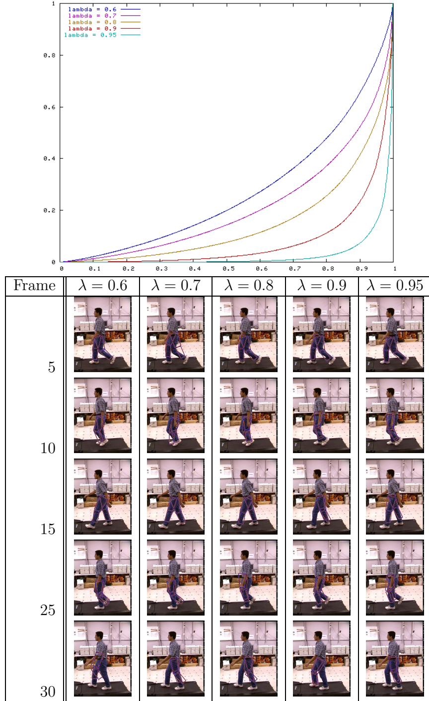
Figure 4.1: Oriented edge tracking results with respect to \lambda : The distributions (top) are plotted according to the specifications in Section 4.2.1. The tracking broke down shortly after frame 30 for \lambda = 0.8 .
