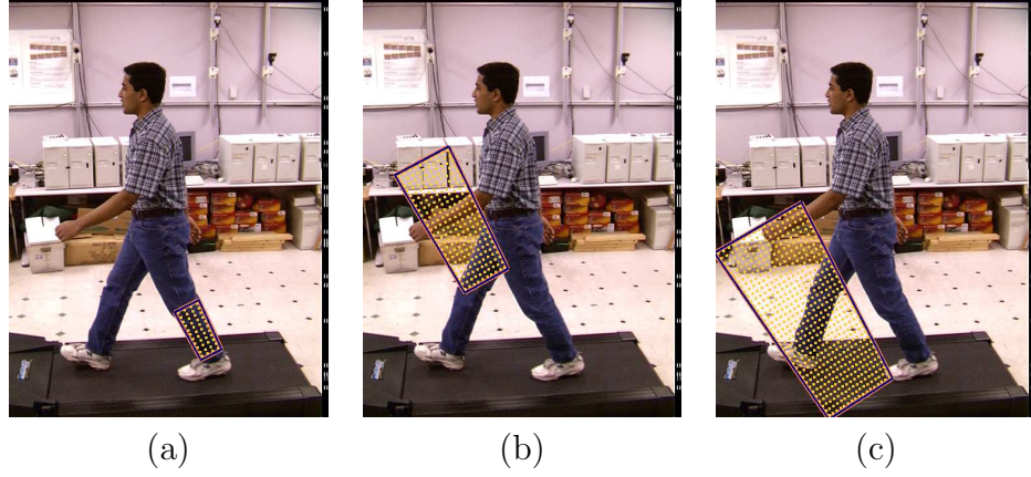
Figure 2.9: The constancy of measurement frequency in two-dimensional image space: Images (a), (b), and (c) show the actual pixel locations of the individual background subtraction sub-measurements for a limb parameterized further and then increasingly closer to the camera. The number of samples taken in the image per unit area is constant.
