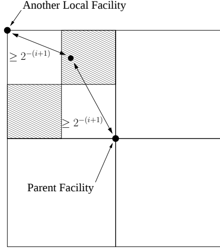
Figure 9: A partition at the (i + 1) -th level
