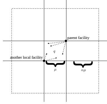
Figure 3: Visualization of Optimal Facility Placement
