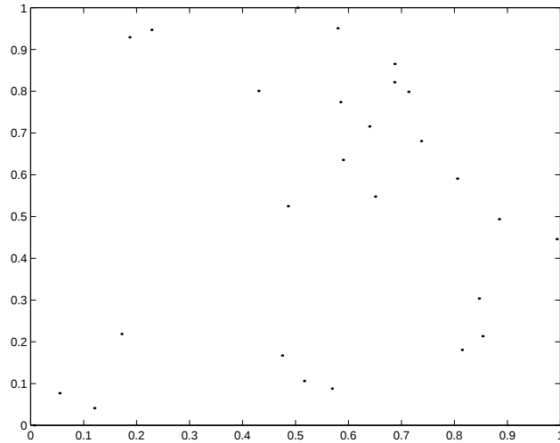
Figure 12: Rhode Island Town Locations
