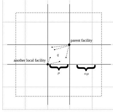
Figure 4: Illustrating Corollary 1. There must exist an optimal facility in the square whose sides have length (2\alpha + 1)\mu .
