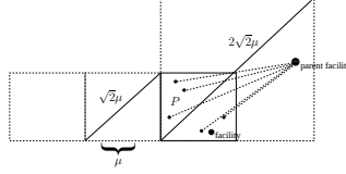
Figure 6: Visualization of Optimal Facility Placement
