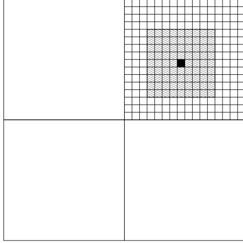
Figure 10: A quadrant of a disjoint bush
