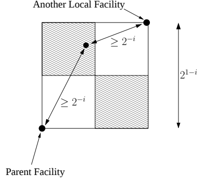
Figure 8: A partition at the i -th level
