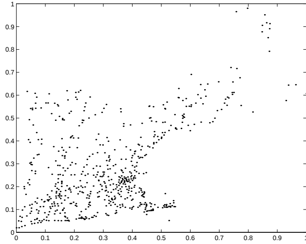
Figure 11: New England Town Locations
