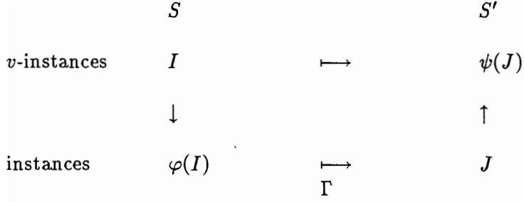
Figure 1: Using IQL for the value-based model
