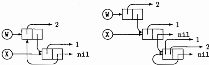
Figure 19. Two possible truncations.
