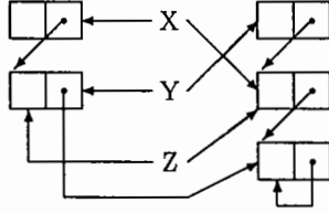
Figure 5. A large, unacceptable merge.
