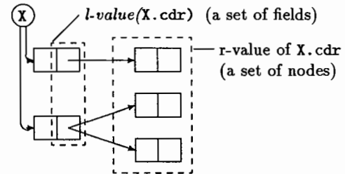
Figure 3. Example of l -value and r -value.
