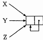
Figure 8. No deterministic variables.
