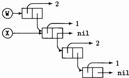
Figure 18. Before summary.
