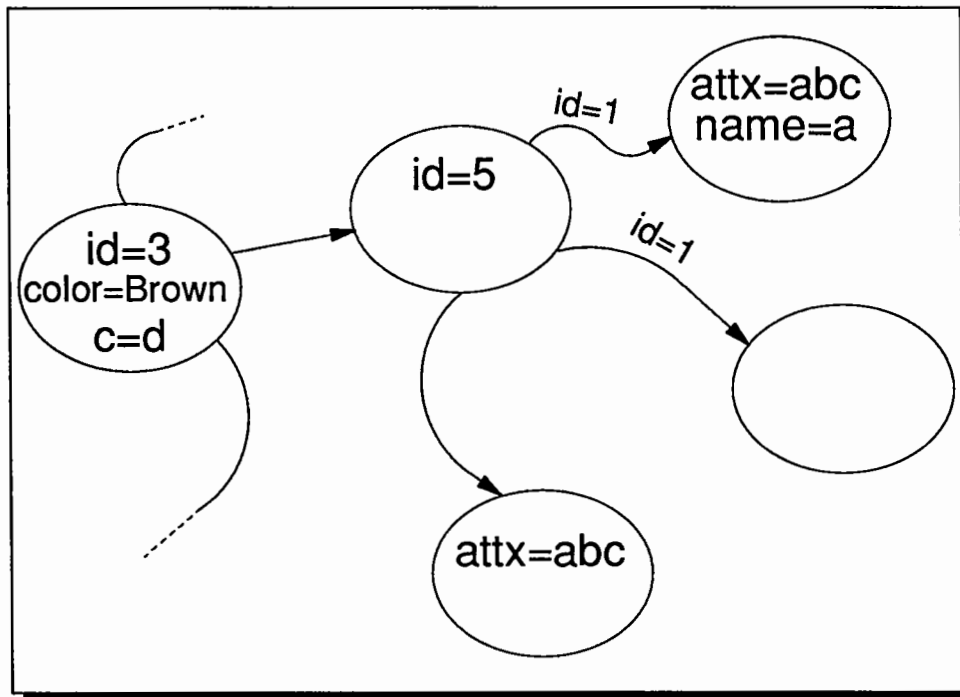
Figure 8 Query example
