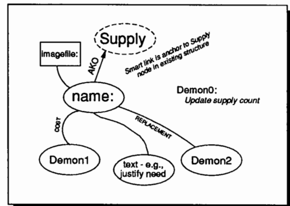
Figure 11 Principled extension of KB through linked templates
