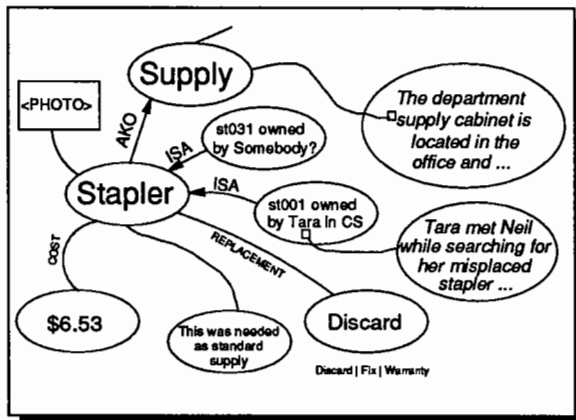
Figure 10 Existing representation for an office supply KB
