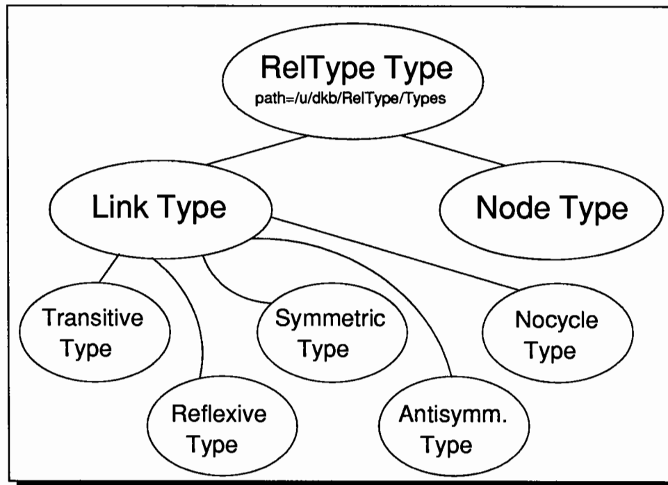
Figure 5 Defined Types type taxonomy
