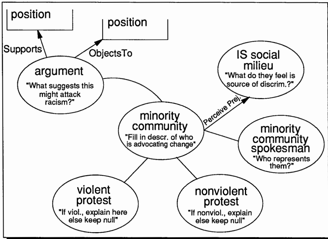
Figure 13 Confrontation template
