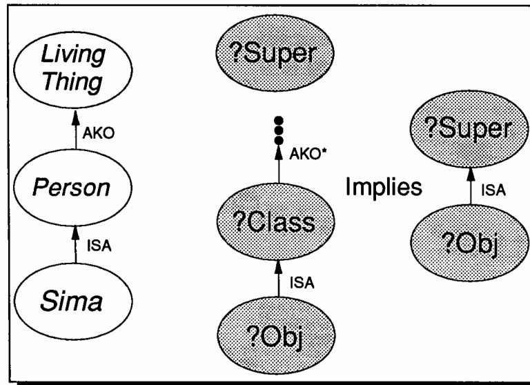
Figure 1 Path-based inference
