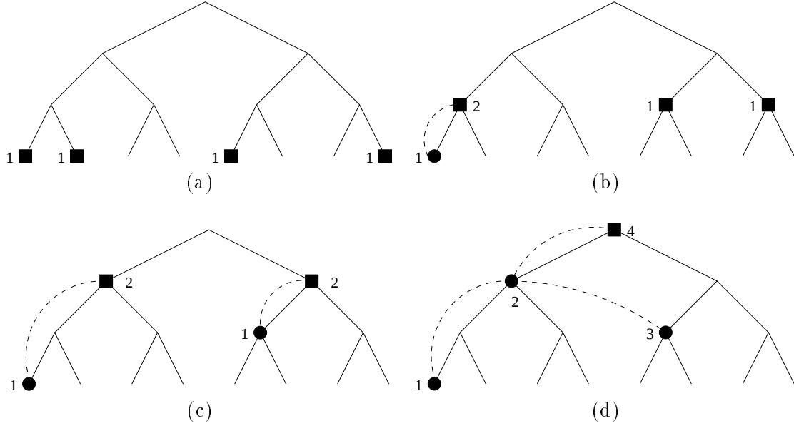
Fig. 11. An illustration of phase E1 with 8 processors of which 4 have failed. Circles indicate processors that have stopped their ascent because of encounters with other live processors and squares indicate processors that continue their upward movement. The numbers beside the processors indicate their ranks at each stage of the algorithm.
