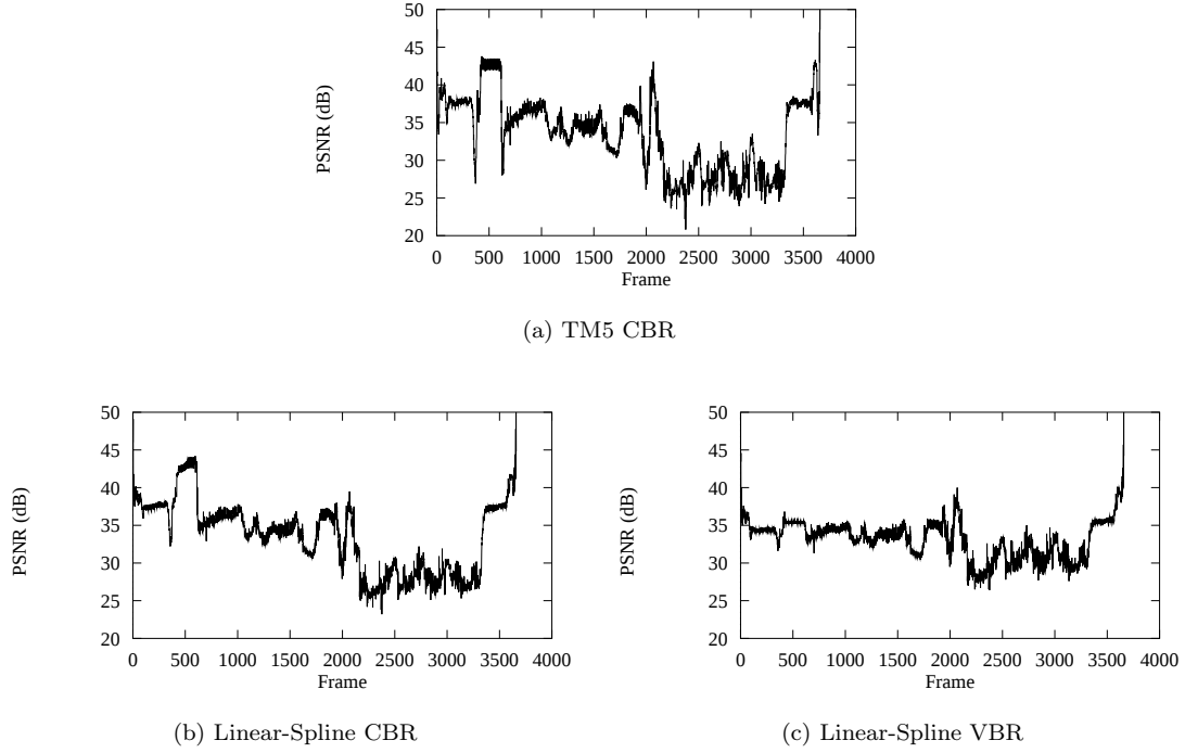
Figure 9.12: PSNR for coding IBM Commercial.
