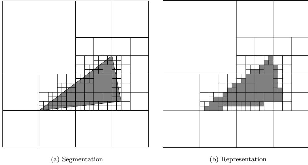
Figure 5.2: Representation of a triangle using a quadtree of depth 5.
