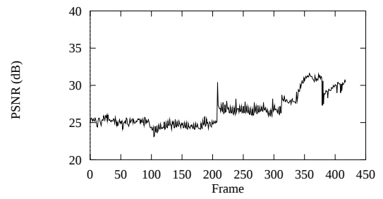
(b) Hyperbolic VBR Pass 2
