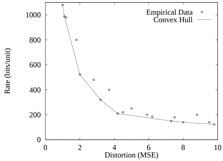
Figure 3.6: Sample operational rate-distortion plot. Plotted is rate versus average distortion.
