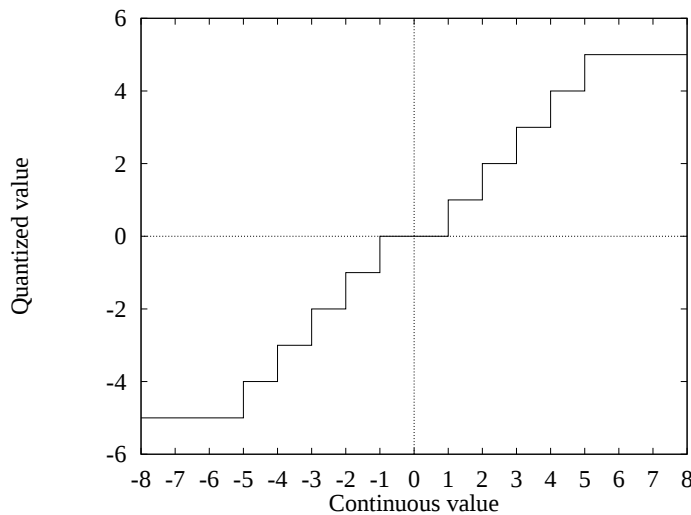
Figure 3.3: Example of uniform quantization.
