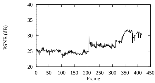
(a) Hyperbolic VBR Pass 1
