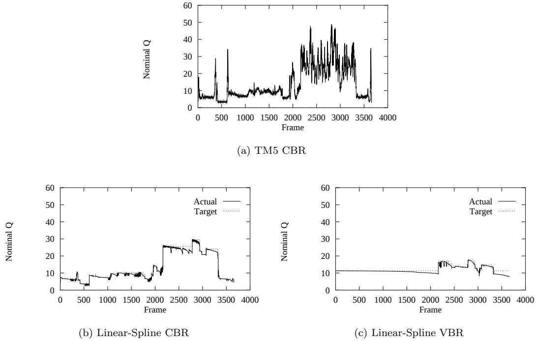
Figure 9.11: Nominal quantization scale for coding IBM Commercial.
