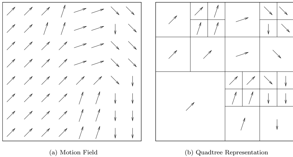
Figure 5.3: Quadtree representation of a motion field.
