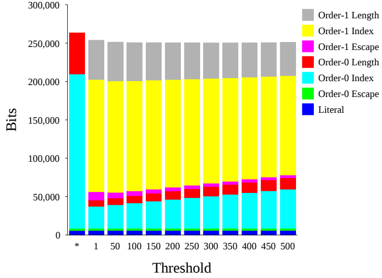
(c) Order-1 LZ77-PM
