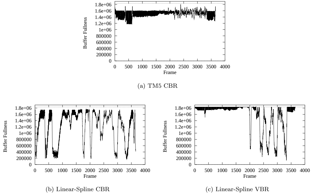
Figure 9.10: Evolution of buffer fullness for coding IBM Commercial.
