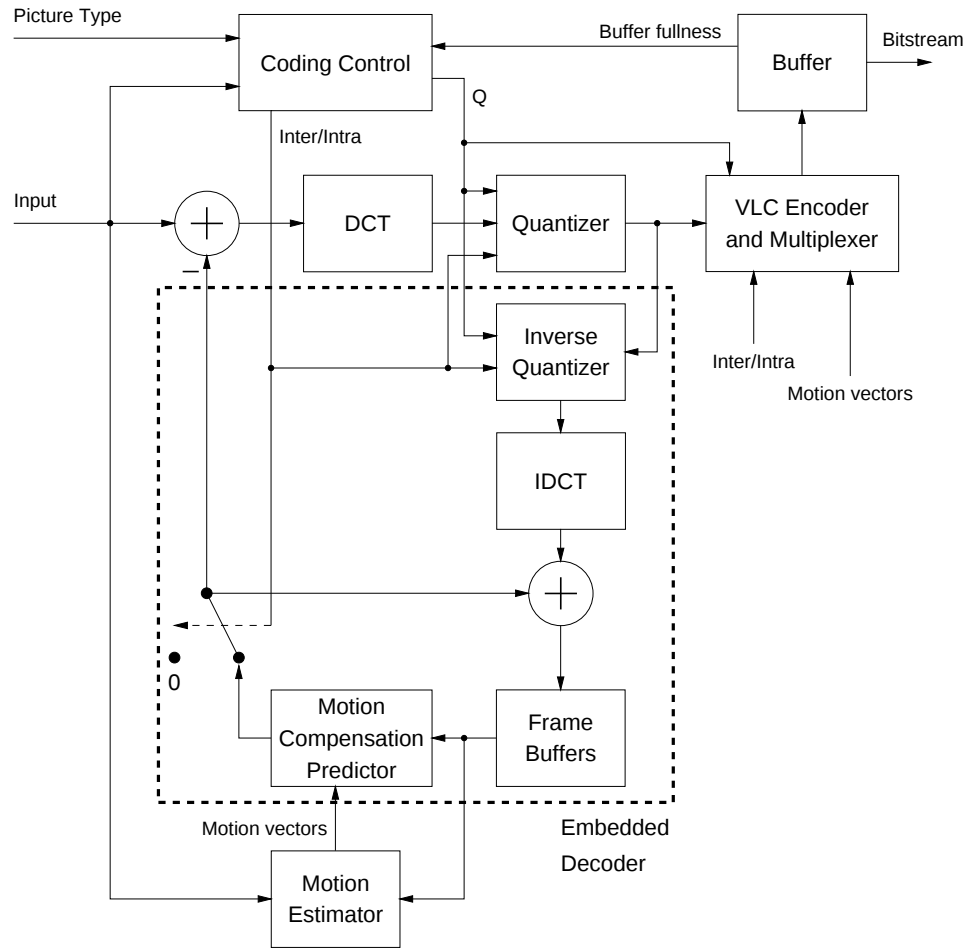
Figure 3.22: Block diagram of a typical MPEG encoder.
