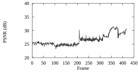
(c) Hyperbolic VBR Pass 3
