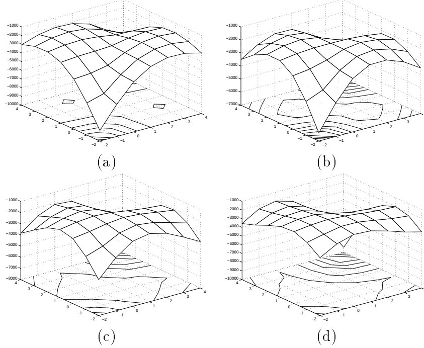
Figure 3: Plots of L(\theta) for 1-dimensional data as a function of \mu_1 and \mu_2 with \alpha_1 = \alpha_2 = 0.5, \sigma_1 = \sigma_2 = 1 . In this case the data is 1000 sampled points from the mixture model with parameters \alpha_1 = \alpha_2 = 0.5, \sigma_1 = \sigma_2 = 1, \mu_1 = 0 and (a) \mu_2 = 3 , (b) \mu_2 = 2 , (c) \mu_2 = 1 , and (d) \mu_2 = 0 . Note how the log likelihood function gets flatter around the maximum as the means in the mixture get closer to each other.
